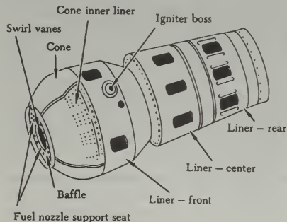
FIGURE 10-58. Combustion chamber liner nomenclature.
